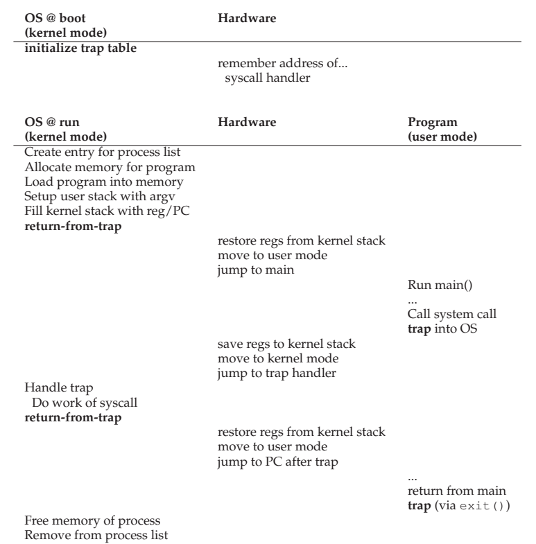
Figure 6.2: Limited Direct Execution Protocol
